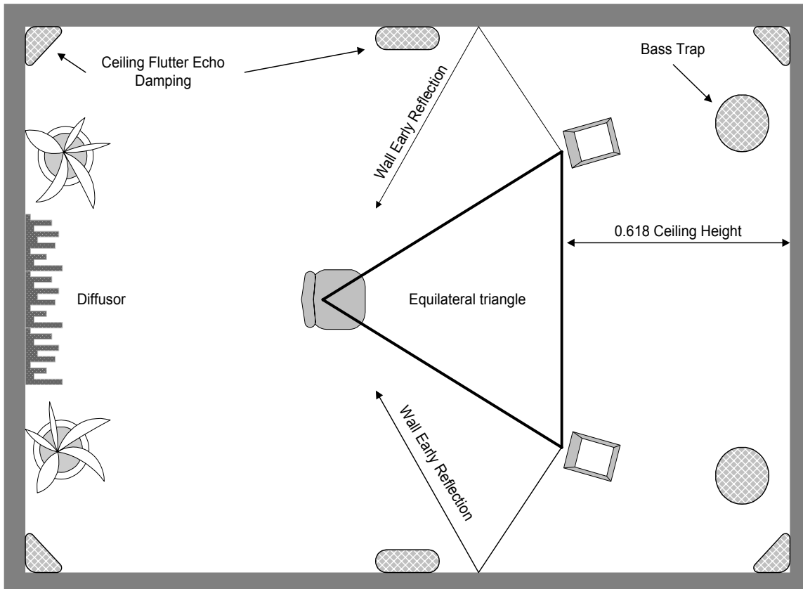
Figure 1: Room placement method no. 1 and different room treatment devices.
